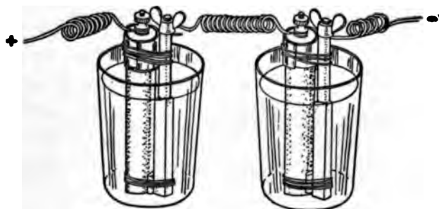
FIG. 204. — Two Home-Made Battery Cells Connected in Series.
